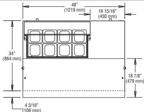
PAN TOP CONFIGURATION
